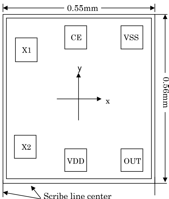
Fig. 7-2 Pad Layout of Cross Type
